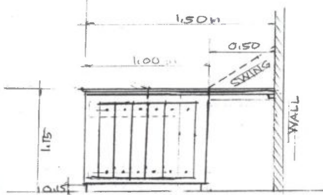
L-SIDE VIEW
