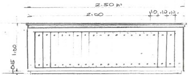
FRONT VIEW
