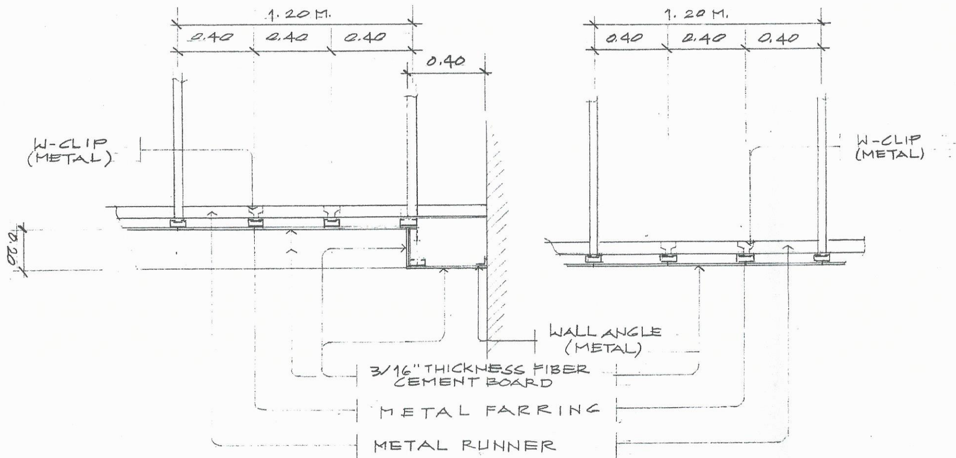
SPOT DETAIL "B"
