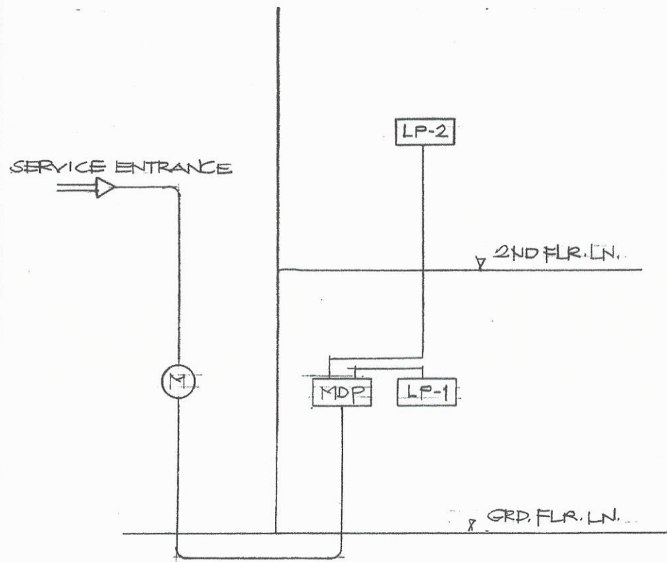
RISER DIAGRAM
