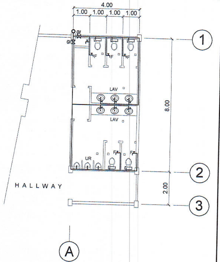
WATER SUPPLY LINE LAYOUT REV. 4TH FLR. CR (NORTH WING) SCALE 1 : 125 MTS.
