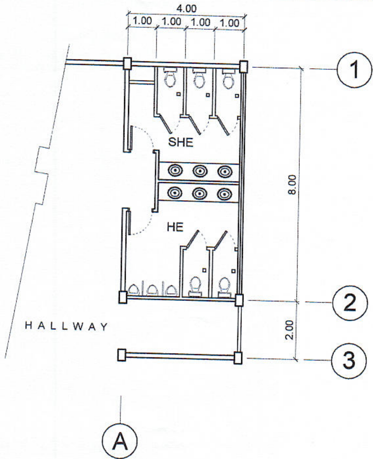
EXISTG. 4TH FLR. CR (NORTH WING) SCALE 1 : 125 MTS.
