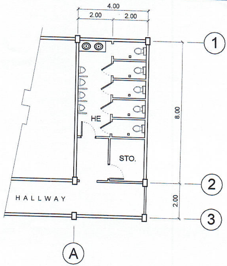
EXISTG. 3RD FLR. BOYS CR (NORTH WING) SCALE 1 : 125 MTS.
