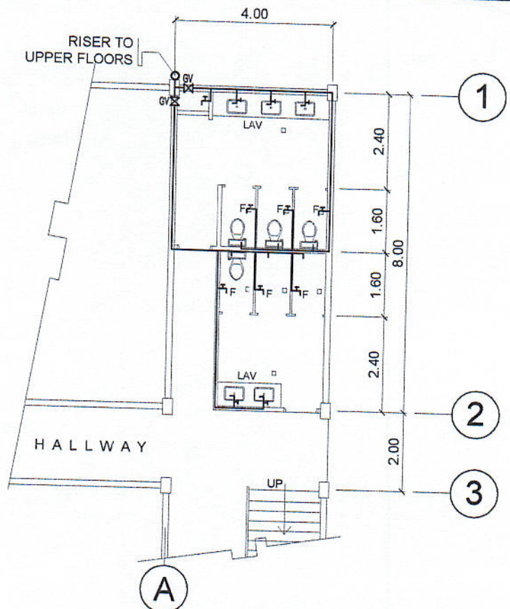
WATER SUPPLY LINE LAYOUT REV. GRD. FLR. FACULTY CR (NORTH WING) SCALE 1 : 125 MTS.
