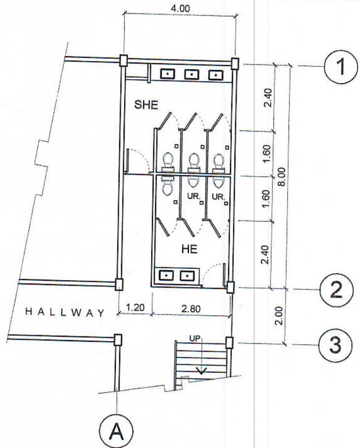
(FOR FACULTY) REV. GRD. FLR. CR (NORTH WING) SCALE 1 : 125 MTS.
