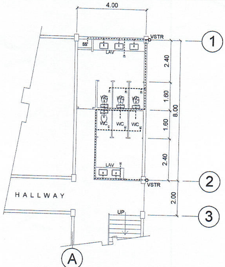
VENTILATION LAYOUT REV. GRD. FLR. GIRLS CR (NORTH WING) SCALE 1 : 125 MTS.
