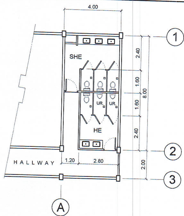
( FOR STUDENTS ) REV. 3RD FLR. CR (NORTH WING) SCALE 1 : 125 MTS.
