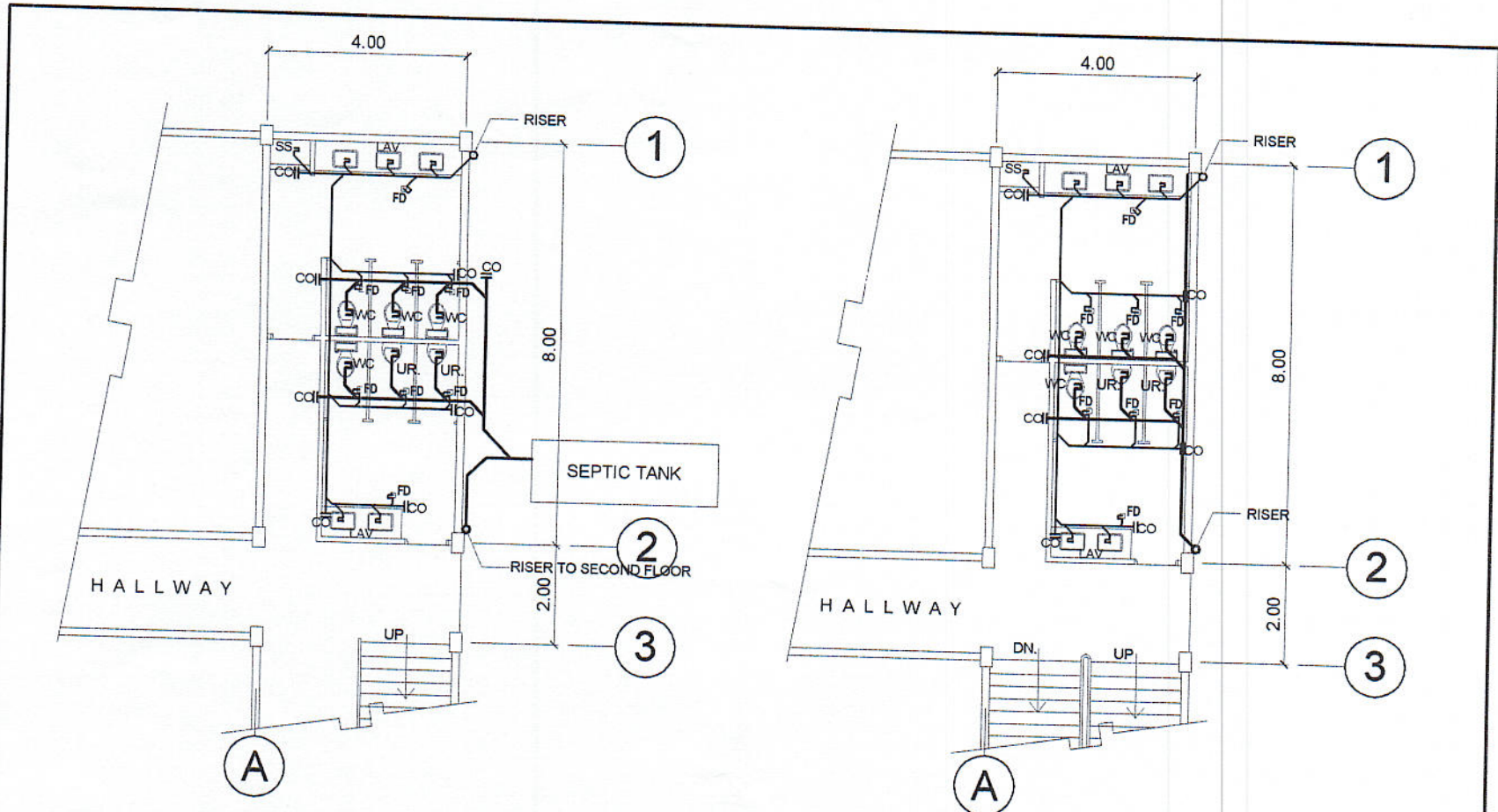
SEWER LINE LAYOUT REV. GRD. FLR. FACULTY CR (NORTH WING) SCALE 1 : 125 MTS.
