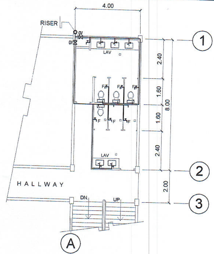
WATER SUPPLY LINE LAYOUT REV. 2ND. FLR. CR (NORTH WING) SCALE 1 : 125 MTS.
