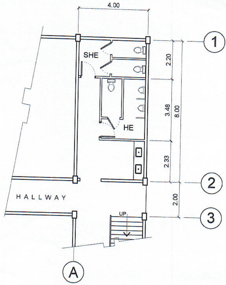
EXISTG. GRD. FLR. CR (NORTH WING) SCALE 1 : 125 MTS.
