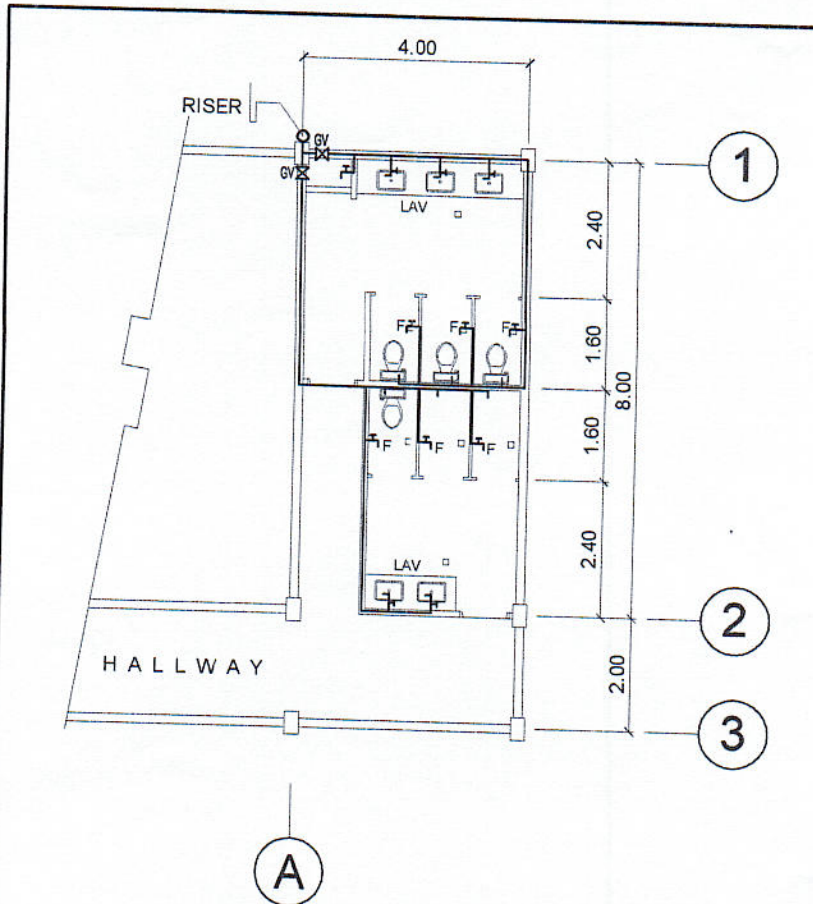
WATER SUPPLY LINE LAYOUT REV. 3RD FLR. CR (NORTH WING) SCALE 1 : 125 MTS.
