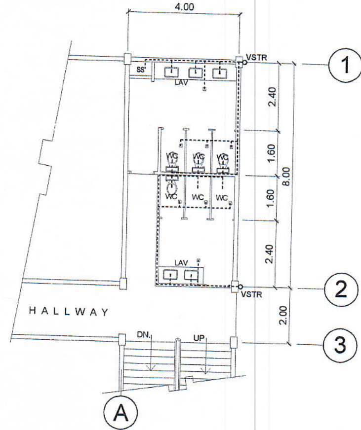
VENTILATION LAYOUT REV. 2ND. FLR. CR (NORTH WING) SCALE 1 : 125 MTS.
