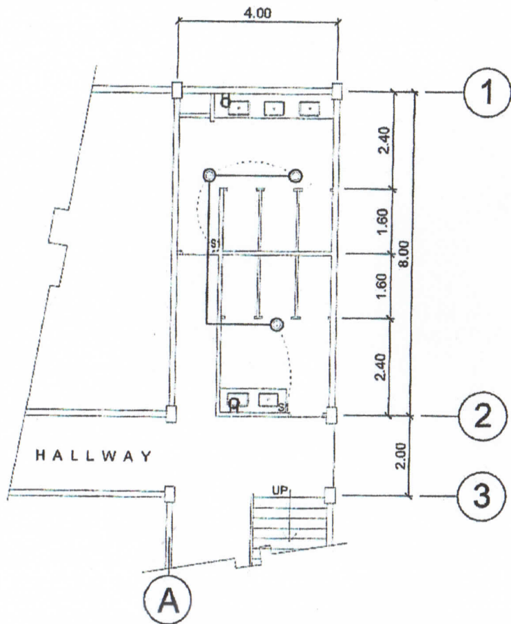
ELECTRICAL LAYOUT REV. GRD. FLR. GIRLS CR (NORTH WING) SCALE 1 : 125 MTS.
