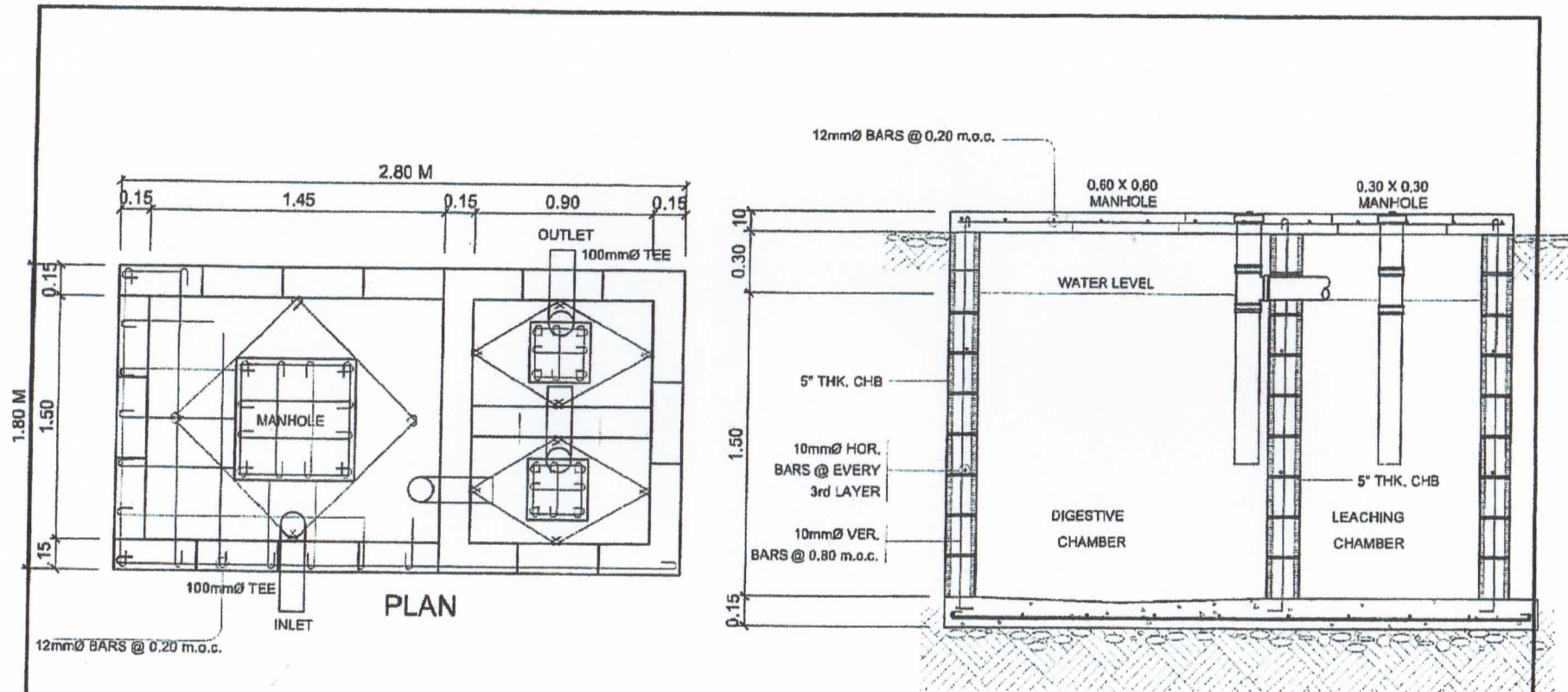
DETAIL OF SEPTIC TANK SCALE 1 : 20 MTS.
