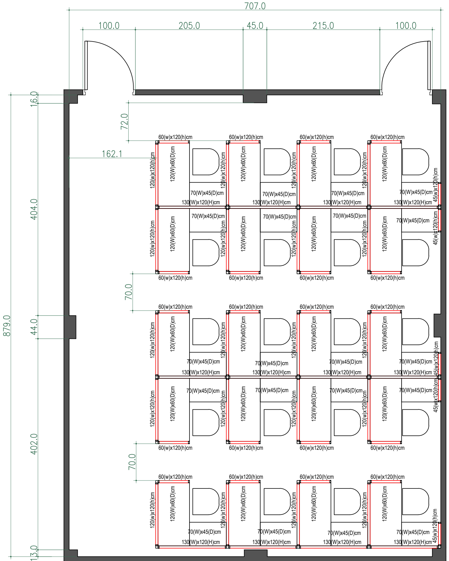
NC207-ECONOMICS PROPOSED FLOOR PLAN SCALE: _____ NTS
