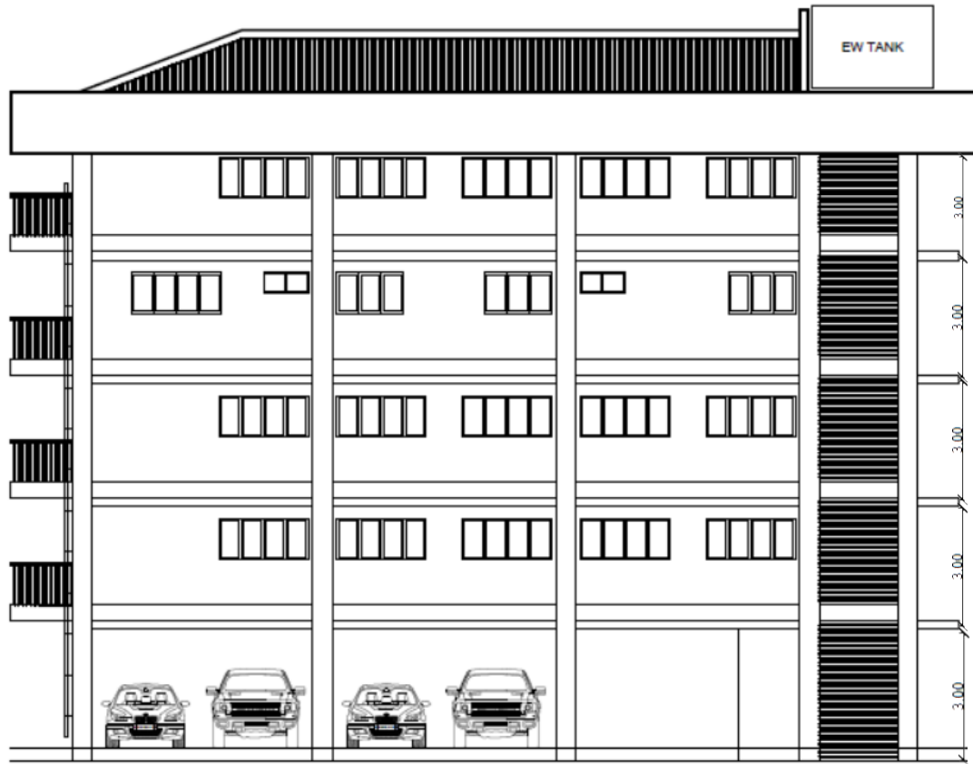
○ PERSPECTIVE PLAN SCALE _____ MTS
