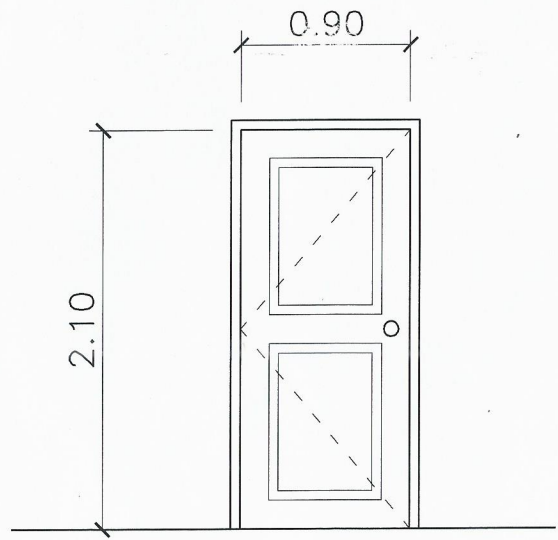
D 1 0.90 X 2.10 STEEL DOOR W/ COMPLETE ACCESSORIES 36 SETS
