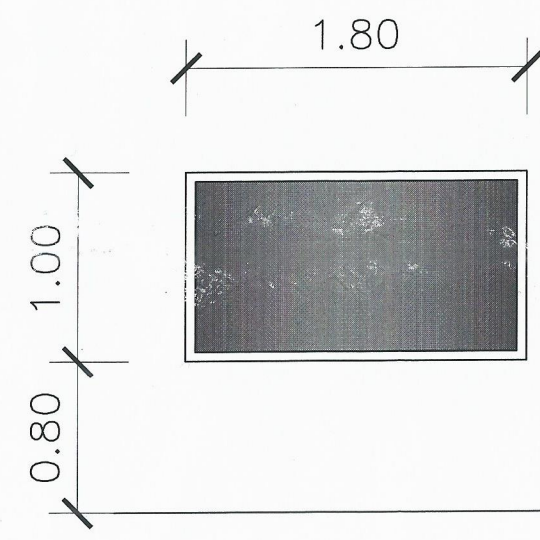
W 1 ALUMINUM FIXED WINDOW COMPLETE W / ALL ACCESSORIES W / \frac{1}{4} " THK CLEAR GLASS 32 SETS
