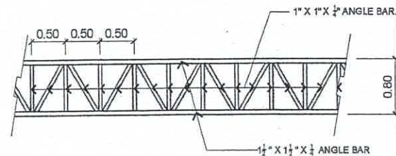
LATERAL FRAME OF GUTTER
