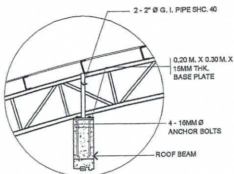
DETAIL "A" SCALE 1: 25 M.
