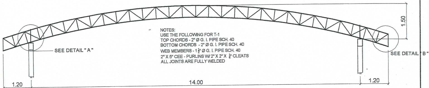
TRUSS DIAGRAM ( TRUSS 1) SCALE 1 : 50M
