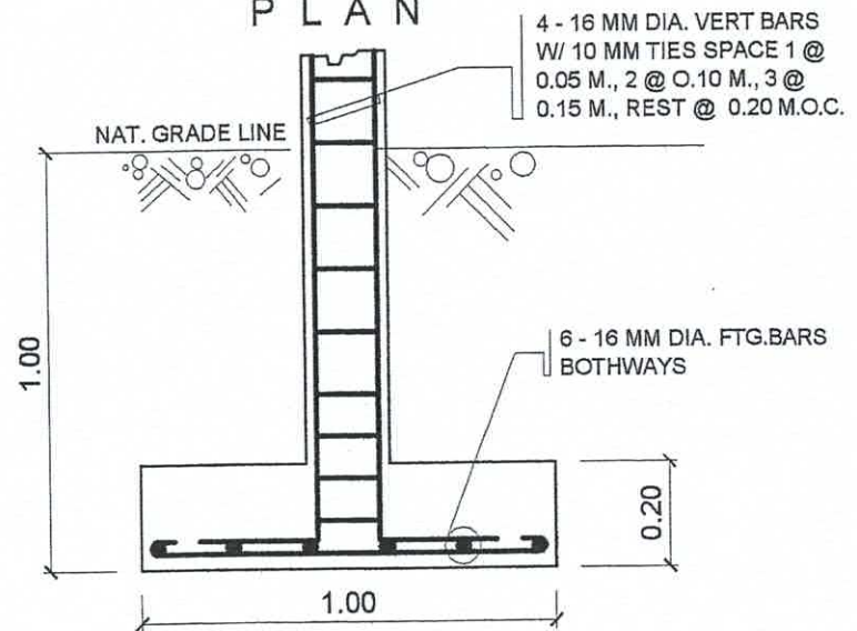
SECTION DETAIL OF C2 - F2
