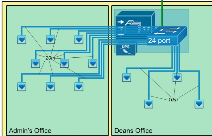
Building 3 (1st Floor)
