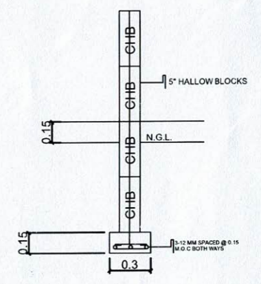
1 A1 SCALE _____ NTS CHB WALL DETAILS
