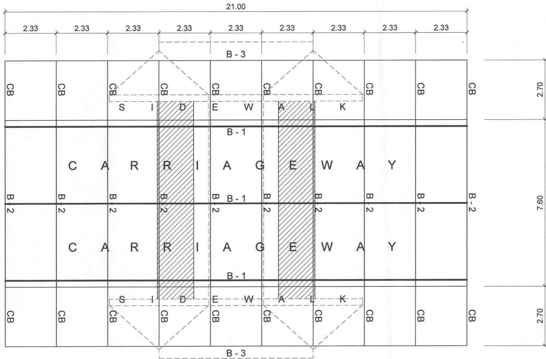
1 S 1 BEAM FRAMING PLAN SCALE 1 : 100 MTS.
