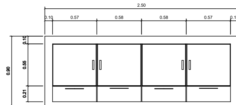
ALUMINUM CABINET DETAILS SCALE NTS
