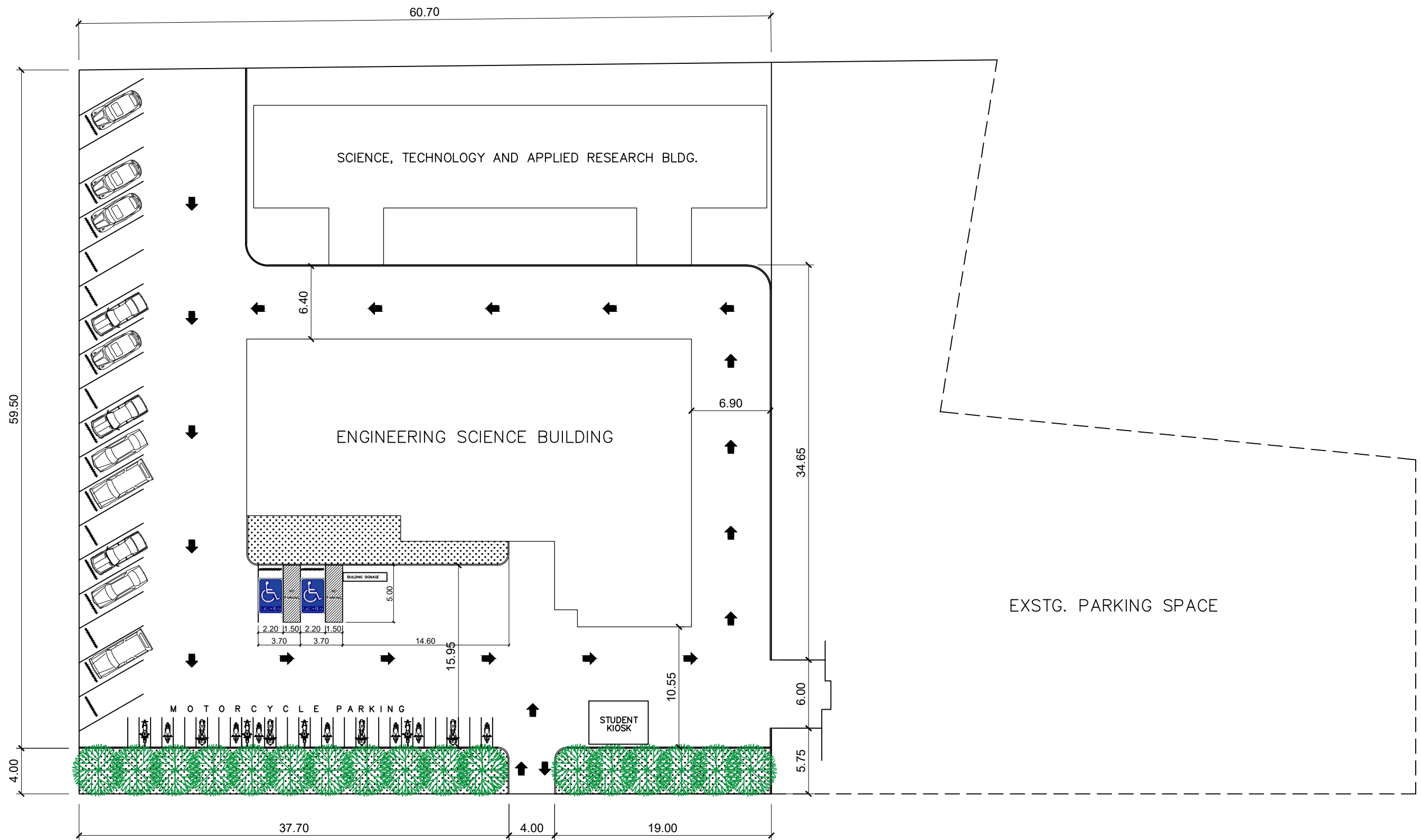
1 SITE DEVELOPMENT PLAN A1 SCALE 1 : 350 MTS.
