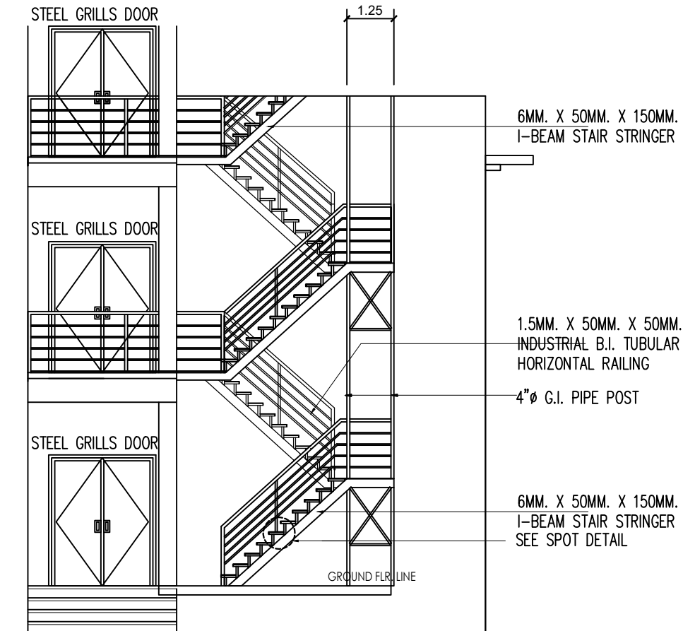
ELEVATION OF FIRE ESCAPE STAIR
