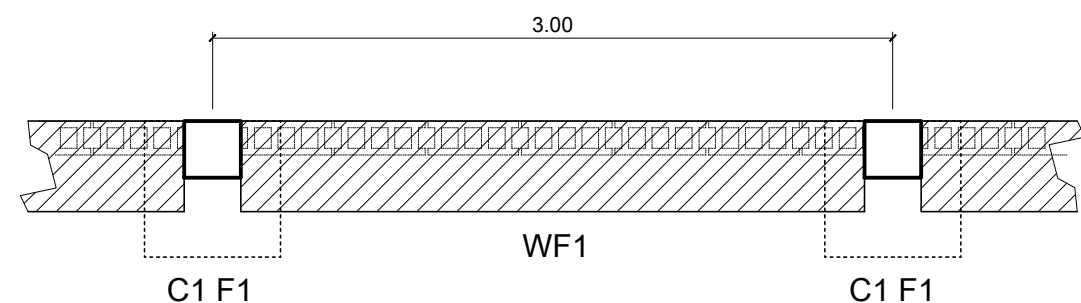
PLAN OF WALL FOOTING
