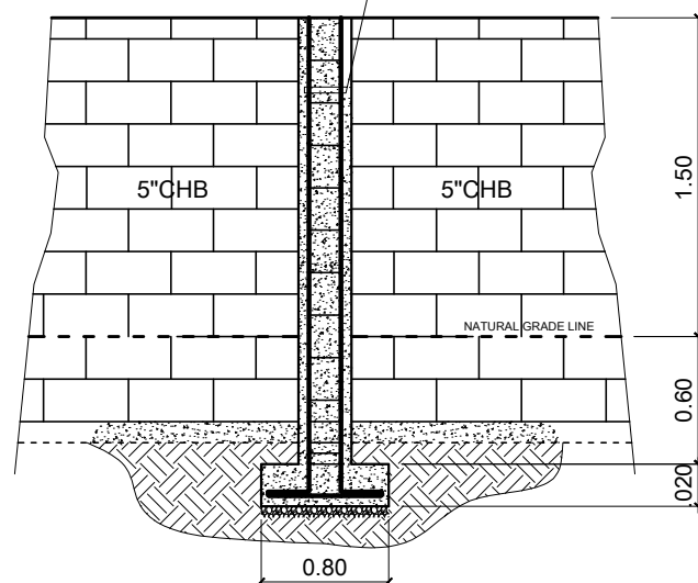
DET.ELEV./ SEC. OF CHB FENCE
